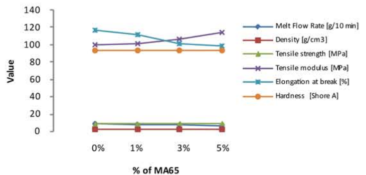
Fig 2 : Effect of properties on Elastoflex ® MA65 of finished product
